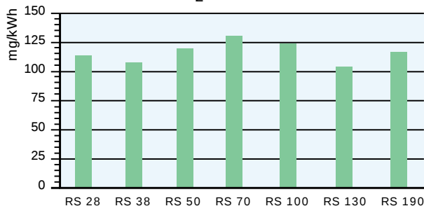
NO 2 EMISSIONS
