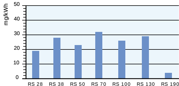
CO EMISSIONS
